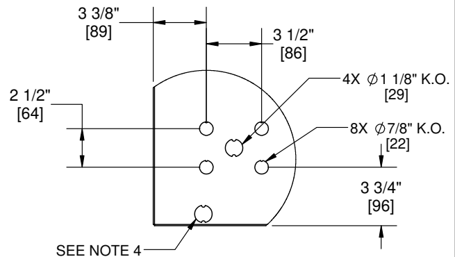
DETAIL D
